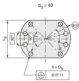
Bohrmuster 2
