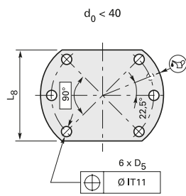
Bohrmuster 1
