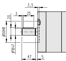
T09xxxxxH25
