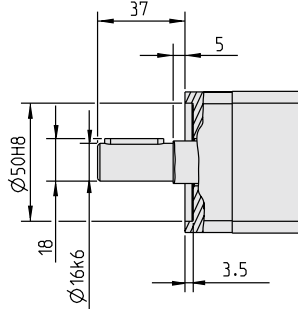
T06xxxxxB25
