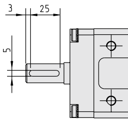
T06xxxxxB/G/H25
