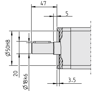
T06xxxxxH25
